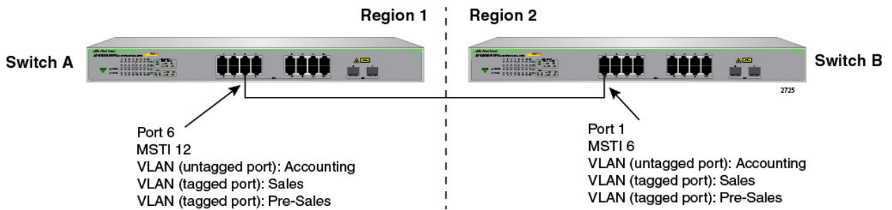
Figure 145. Spanning Regions without Blocking
